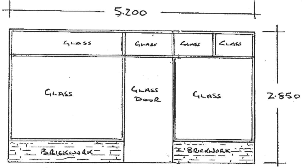
EXISTING DETAIL
